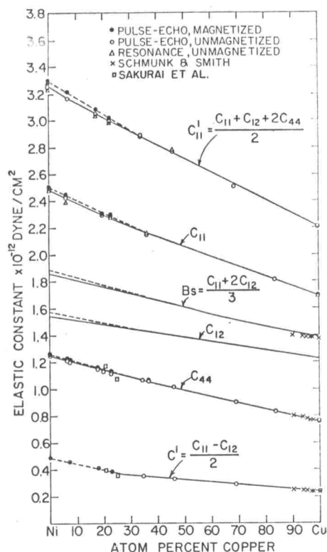
Fig. 2. The elastic constants of nickel-copper alloy single crystals in the magnetically saturated and unmagnetized states.
